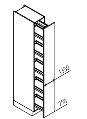
VVA Vorratsschrank ↔ 30/40 ↓ 195/210/225 ↶ 60
