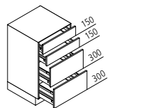
USA Schubkastenschrank ↔ 30/40/45/50/60/80/90/100/120 ↓ 90 ↙ 60/50/39
