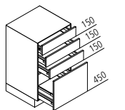
UAS Schubkastenschrank ↔ 30/40/45/50/60/80/90/100 ↓ 90 ↙ 60/50/39
