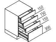
USA Schubkastenschrank ↔ 30/40/45/50/60/80/90/100/120 ↓ 75 ↙ 60/50/39
