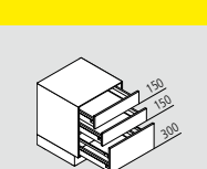
USA Schubkastenschrank ↔ 30/40/45/50/60/80/90/100 ↓ 60 ↙ 60/50
