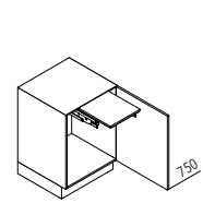
UBKOD Brotmaschinenschrank ↔ 45/50/60 ↓ 75 ↙ 60
